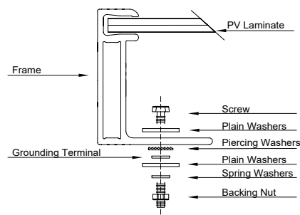
Figure 9: Grounding screw assembly detail
