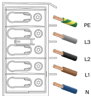
TN/TT 3-phase (3X 230V/400V)
