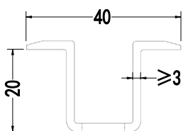
Figure 10: Detail of a clamp
