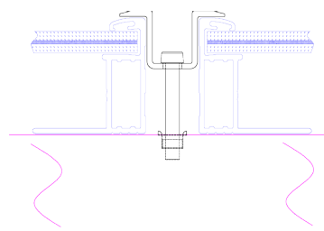
Figure 13: Tighten clamp
