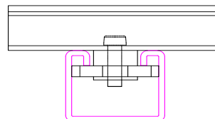
Figure 12: Primary fixation clamp
