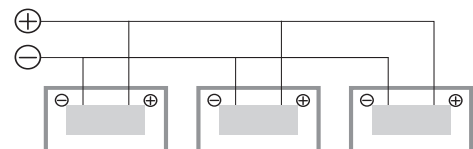
Figure 5: Electrical diagrams of series and parallel wiring
