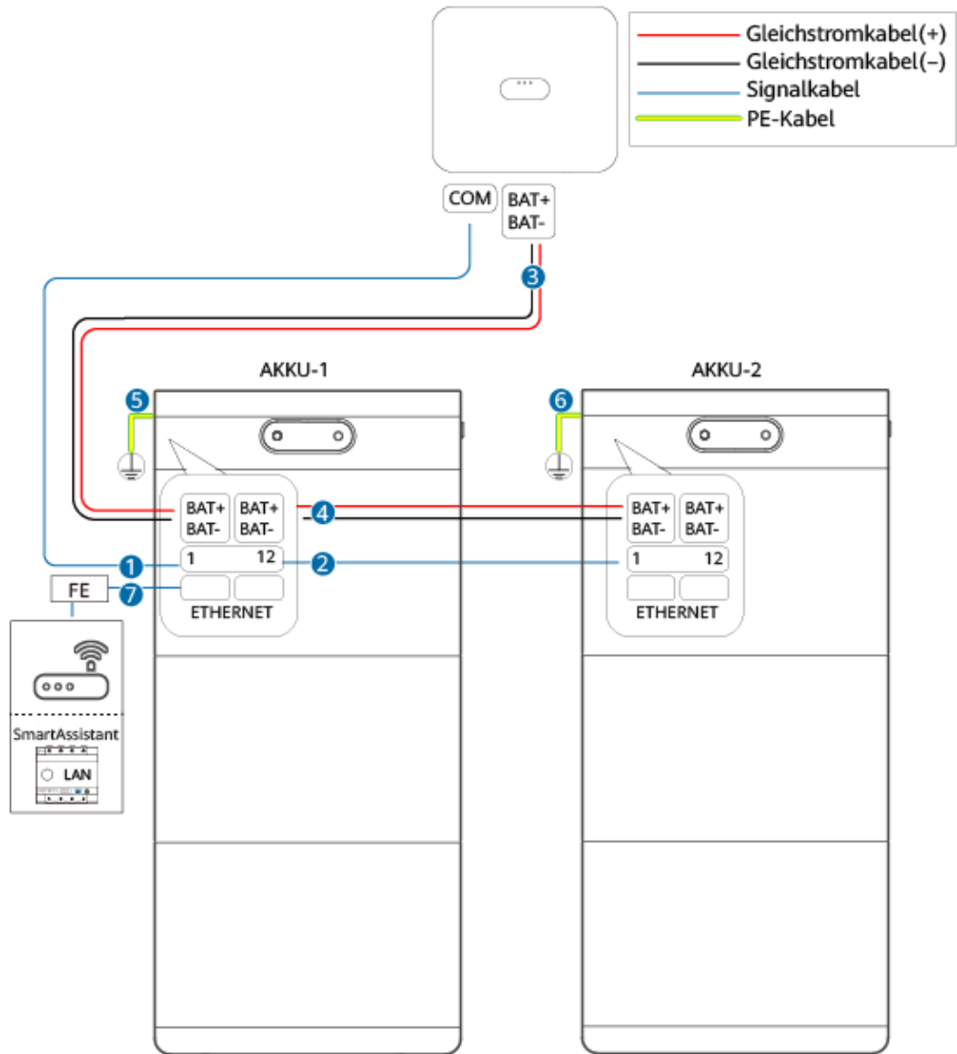
Abbildung 5-1 ESS-Kabelanschlüsse
