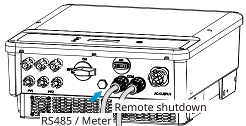
Remote shutdown RS485 / Meter
