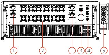
GW73KLV-HT/GW110K-HT/GW120K-HT/GW136K-HTH Unterseite
