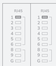
Ideal connection
