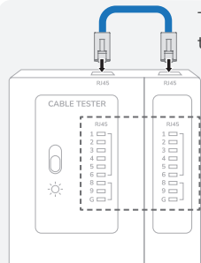
Ethernet Cable Tester
